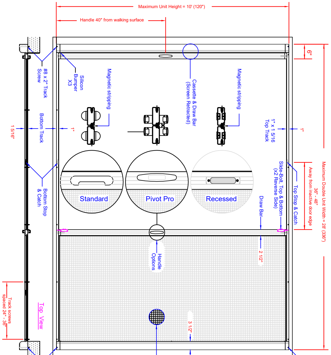
Front View - Double Screen
